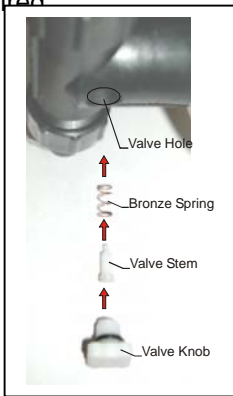
Photo above shows detail of vacuum relief valve for foam bottle. The vacuum relief valve knob does not change the concentration of foam, it only keeps the foam bottle from collapsing as the foam is drawn from it.
